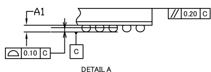
DETAIL A
