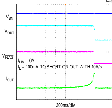
CURRENT-LIMIT RESPONSE
