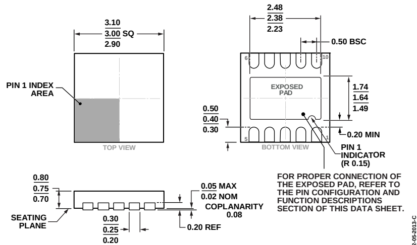
Figure 63. 10-Lead Lead Frame Chip Scale Package [LFCSP_WD] 3 mm x 3 mm Body, Very Very Thin, Dual Lead (CP-10-9)
