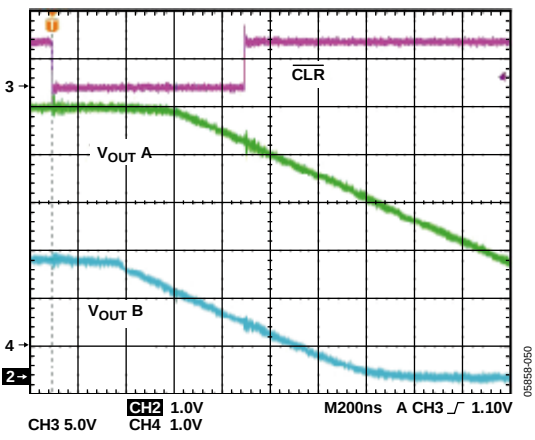
Figure 48. \overline{\text{CLR}} Pulse Activation Time
