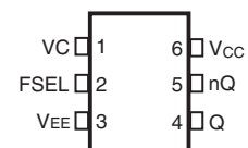
IDT8N3DV85 6-lead ceramic 5mm x 7mm x 1.55mm package body CD Package Top View
