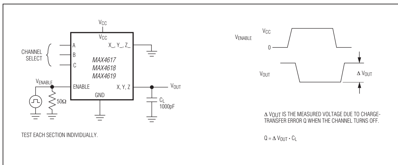
Figure 5. Charge Injection
