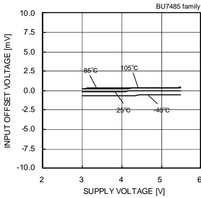
Fig.105 Input Offset Voltage – Supply Voltage (Vicm=VDD-1.4[V], VOUT=1.5[V])
