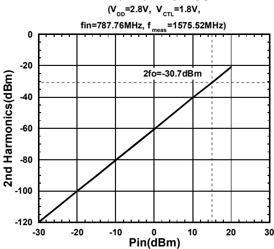
2nd Harmonics
