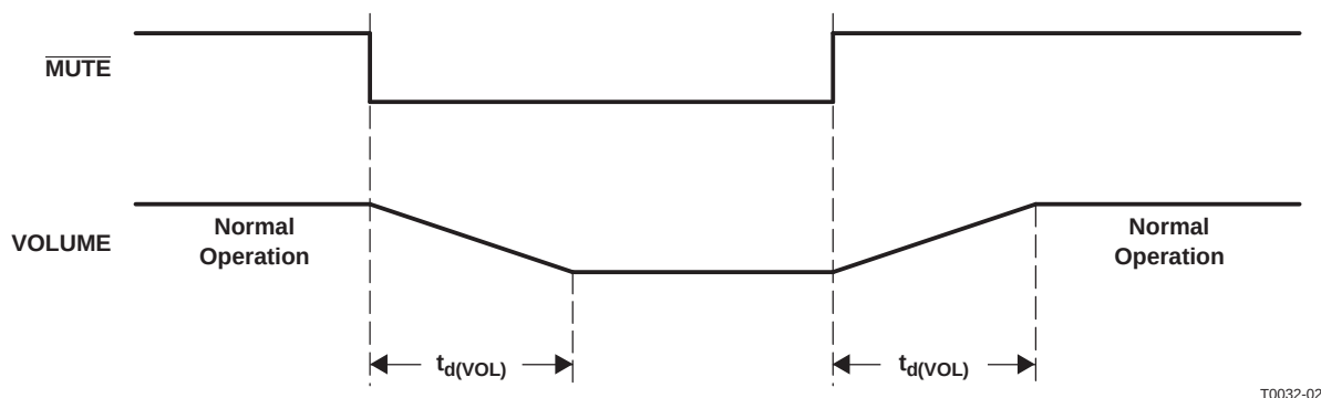
Figure 3-8. Mute Timing
