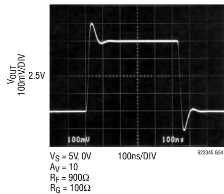
Small-Signal Response
