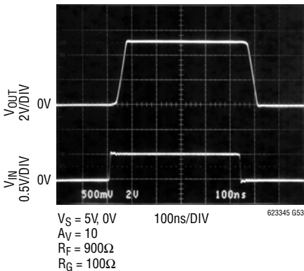
Output-Overload Recovery
