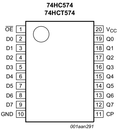
Fig 5. Pin configuration SO20, SSOP20 and TSSOP20
