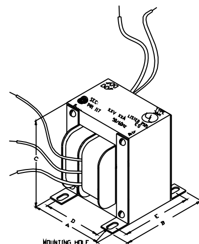
Dimension Table
