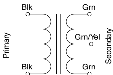
Transformer Schematic
