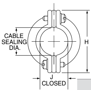
SADDLE CLAMP
