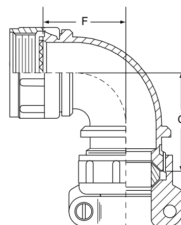
90° ENTRY ROTATABLE COUPLING 2M380MA137
