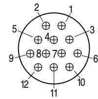
14-12, 16-12, 18-12 (12) #16 Contacts
