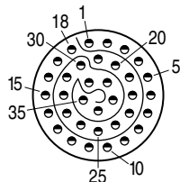
14-235, 16-235, 18-235 (35) #20HD Contacts .023 Max. Dia. Tail
