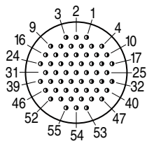
14-55, 16-55, 18-55 (55) #23 Contacts .022 Max. Dia. Tail
