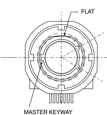
8-13 MASTER KEYWAY LOCATION
