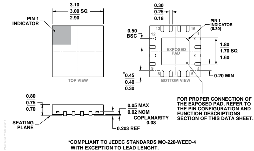
Figure 33. 16-Lead Lead Frame Chip Scale Package [LFCSP] 3 mm x 3 mm Body and 0.75 mm Package Height (CP-16-33) Dimensions shown in millimeters
