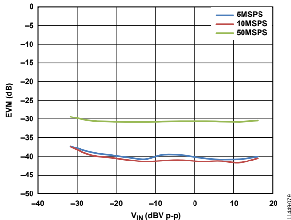
Figure 73. EVM vs. Input Voltage over Symbol Rates; Filter Corner = 63 MHz, QPSK, Gain Code = 0000000, 1.5 V p-p Differential Output Level Maintained
