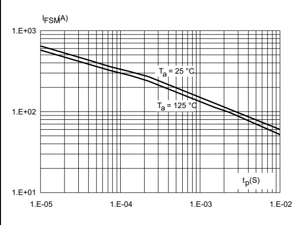
Figure 7. Non-respective peak surge forward current versus pulse duration (sinusoidal waveform, per diode)
