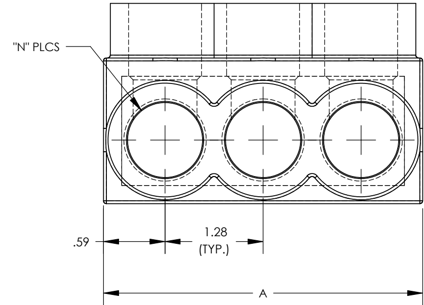
THREE PORT CONNECTOR BLOCK SHOWN WITH PLASTIC CLOSURE PLUGS REMOVED. SEE TABLE FOR DIMENSIONS OF PARTS WITH ADDITIONAL PORTS
