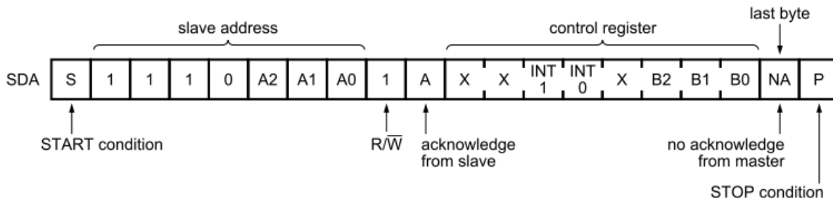
Figure 12. Read Control Register
