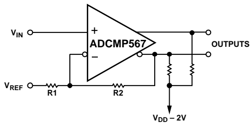
Figure 9. Hysteresis Using Positive Feedback
