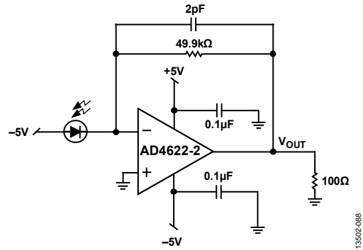
Figure 87. Photodiode Preamplifier
