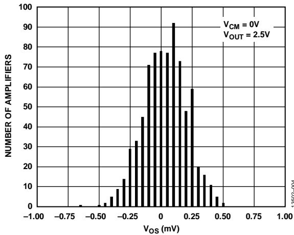
Figure 7. Input Offset Voltage ( V_{OS} ) Distribution, V_{SY} = 5 V
