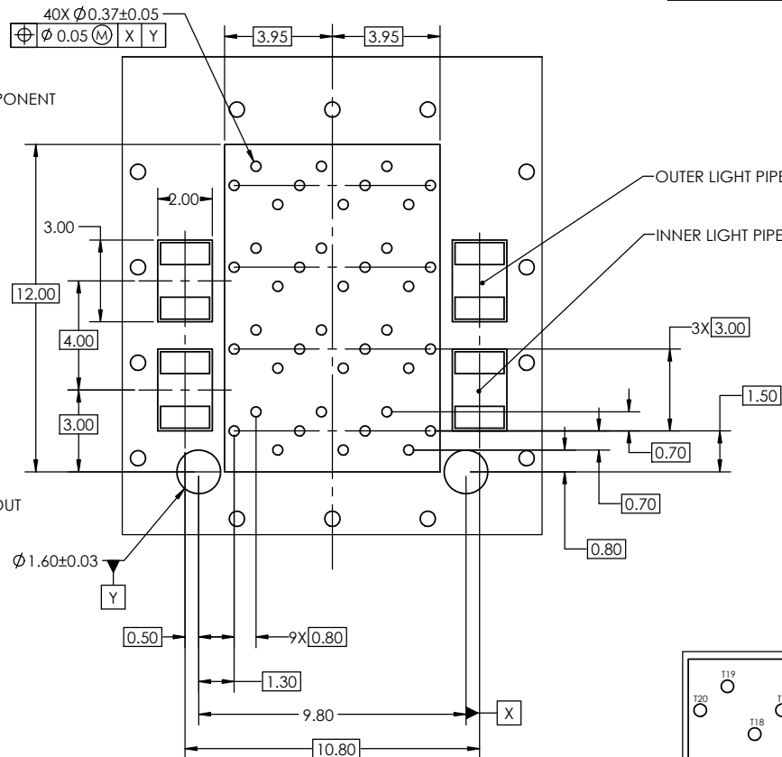
DETAIL C: SCALE 8 : 1
