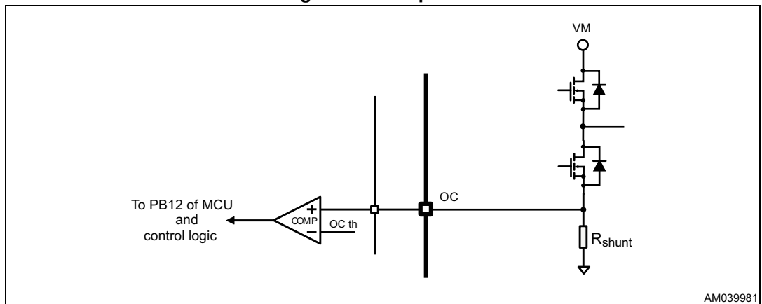
Figure 15. Comparator
