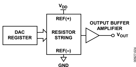
Figure 24. DAC Channel Architecture
