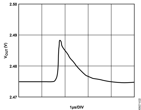
Figure 22. Major-Code Transition
