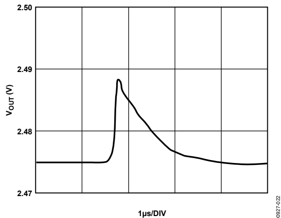
Figure 22. Major-Code Transition
