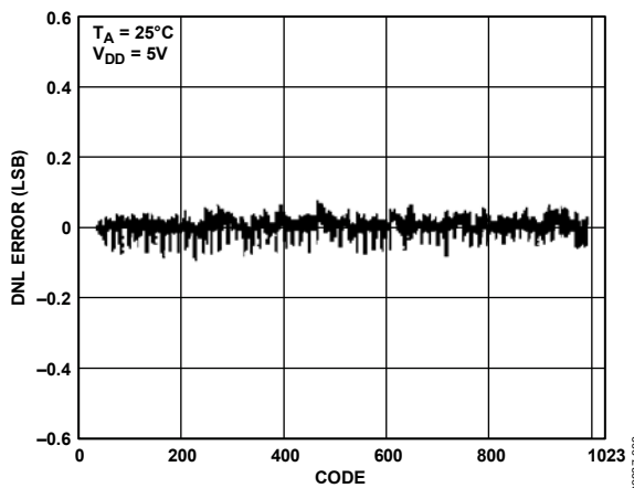
Figure 9. AD5311 Typical DNL Plot
