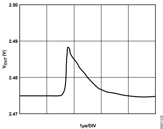
Figure 22. Major-Code Transition
