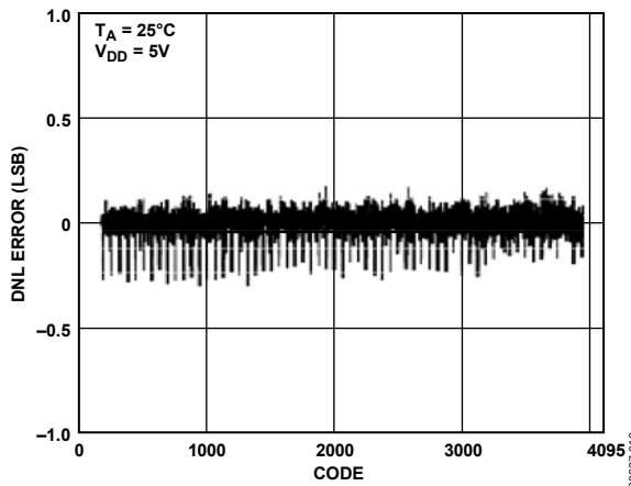
Figure 10. AD5321 Typical DNL Plot
