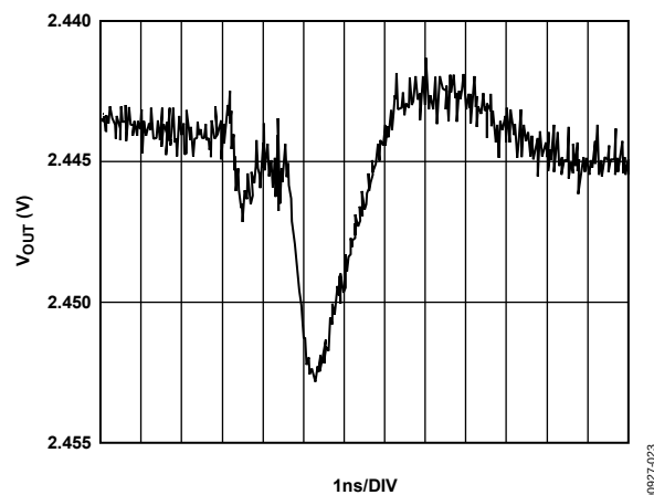
Figure 23. Digital Feedthrough
