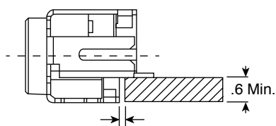
Mount Position: Within .15mm from P.C.B edge
