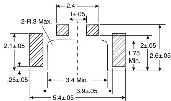
P.C.B Layout (View from the direction A)
