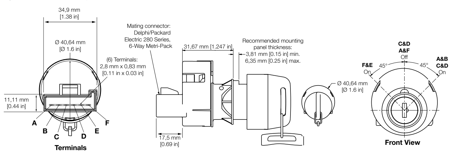
Figure 5. Model 89680 Key Switch Dimensions
