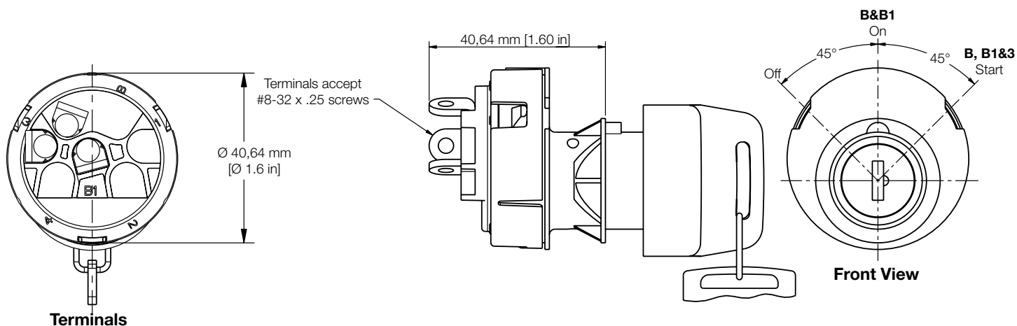
Figure 10. Model 84829 Key Switch Dimensions
