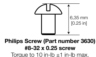
Figure 14. Screw Dimensions
