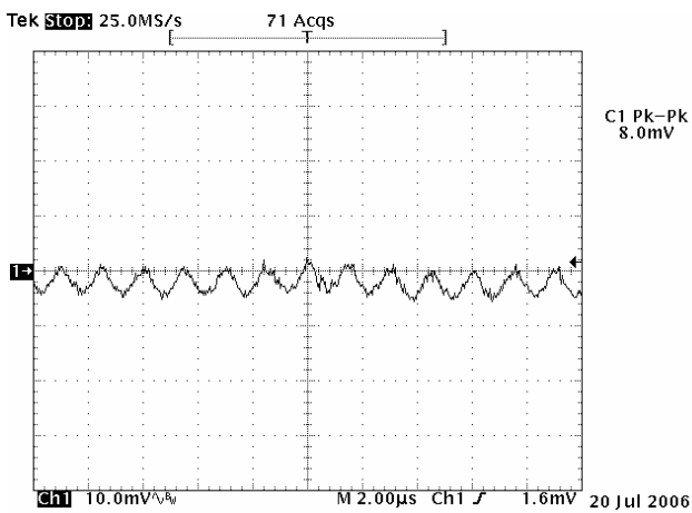
Figure 9: Output Ripple & Noise ( V_{in}=12V , V_{out}=1.5V/10A , Environment Temp.=25°C)
