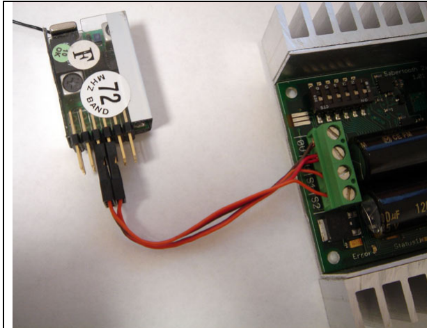
Figure 5.1: R/C connection
