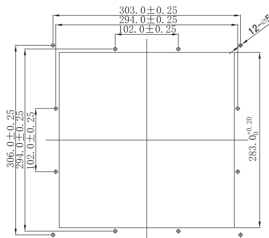
PANEL CUTOUT
