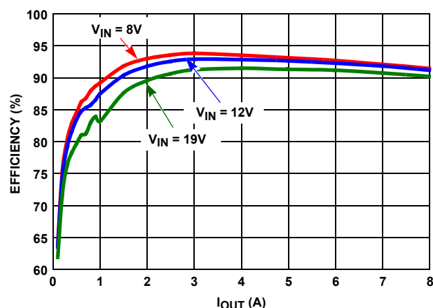
FIGURE 9. CHANNEL 1 EFFICIENCY AT V_O = 1.5V
