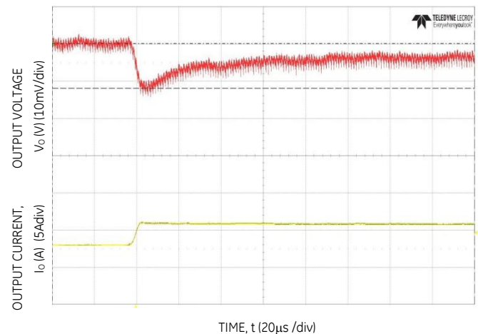
Figure 4. Transient Response to Dynamic Load Change from 50% to 100% at 12V in , C out =3x47μF+3x330μF, C Tune =10nF, R Tune =300Ω
