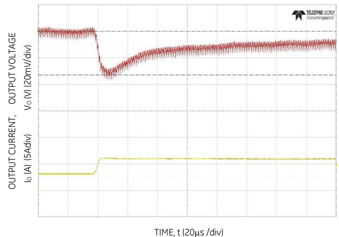
Figure 16. Transient Response to Dynamic Load Change from 50% to 100% at 12Vin, C_{out}=3 \times 47\mu\text{F} + 1 \times 330\mu\text{F} , C_{Tune}=3900\text{pF} , R_{Tune}=300
