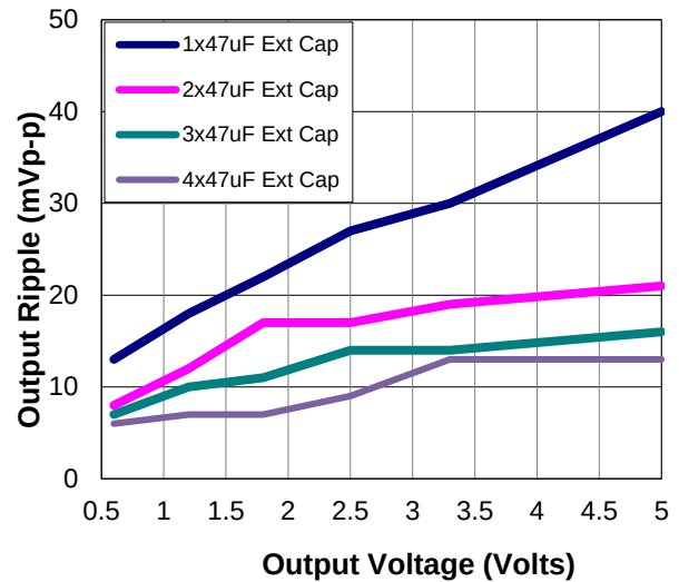
Figure 38. Output ripple voltage for various output voltages with external 1x47 \mu F, 2x47 \mu F, 3x47 \mu F, or 4x47 \mu F ceramic capacitors at the output (6A load). Input voltage is 12V. Scope BW Limited to 20MHz
