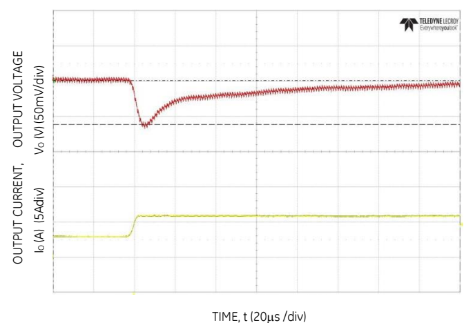
Figure 28 Transient Response to Dynamic Load Change from 50% to 100% at 12Vin, C_{out}=5 \times 47\mu\text{F} , C_{Tune}=1800\text{pF} , R_{Tune}=300
