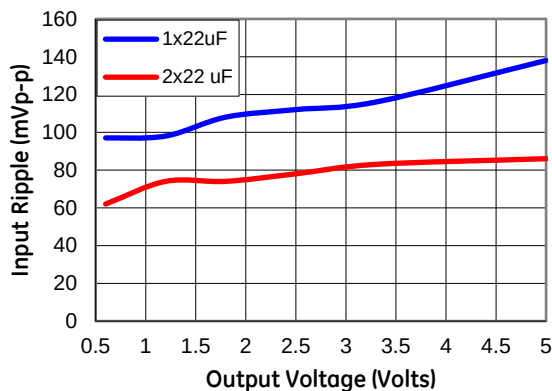
Figure 37. Input ripple voltage for various output voltages with 1x22 \mu F or 2x22 \mu F ceramic capacitors at the input (6A load). Input voltage is 12V. Scope BW Limited to 20MHz
