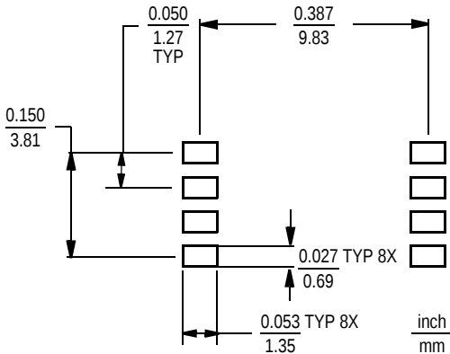
Figure 9. SSOP footprint
