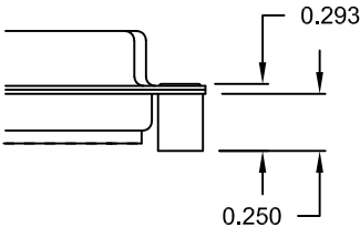
03X..... 0.250" (MATING SIDE) - CN8
