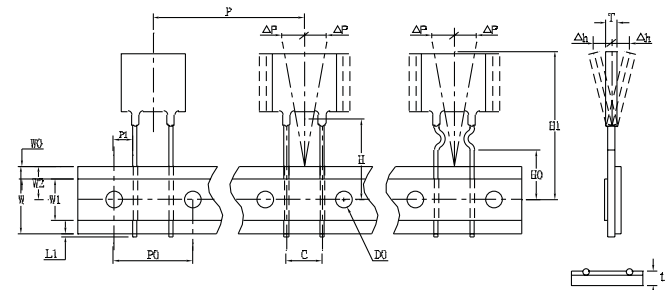
Style 2 - PTR016V1200-PTR016V1500
