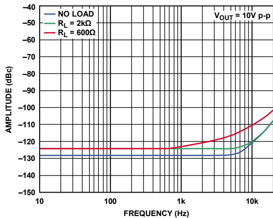
Figure 57. Third Harmonic Distortion vs. Frequency ( G = 1 )
