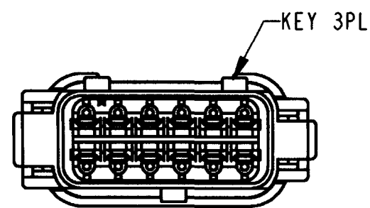
DTM06-12SD-E003 KEY -D- COLOR: BROWN
