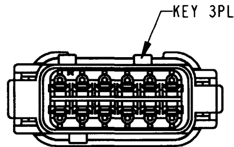
DTM06-12SA-E003 KEY -A- COLOR: GREY
