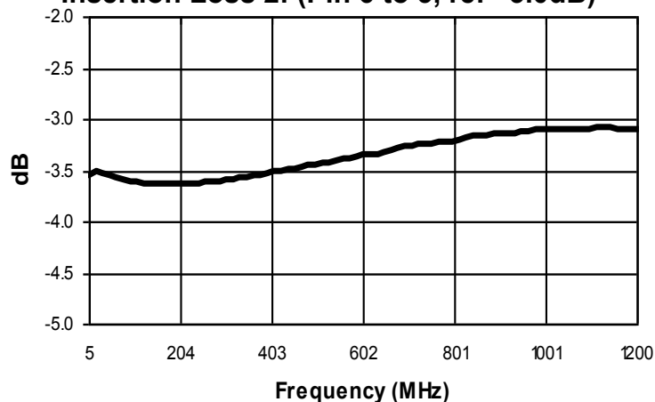
Insertion Loss 2: (Pin 6 to 3, ref -3.0dB)
