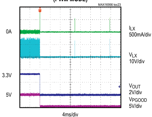
SHORT-CIRCUIT RESPONSE (PWM MODE)
