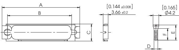
Dimensions Slide Lock Frame F-GV and Fixing Screws
