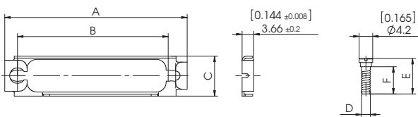
Dimensions Slide Lock Frame F-GV and Fixing Screws
