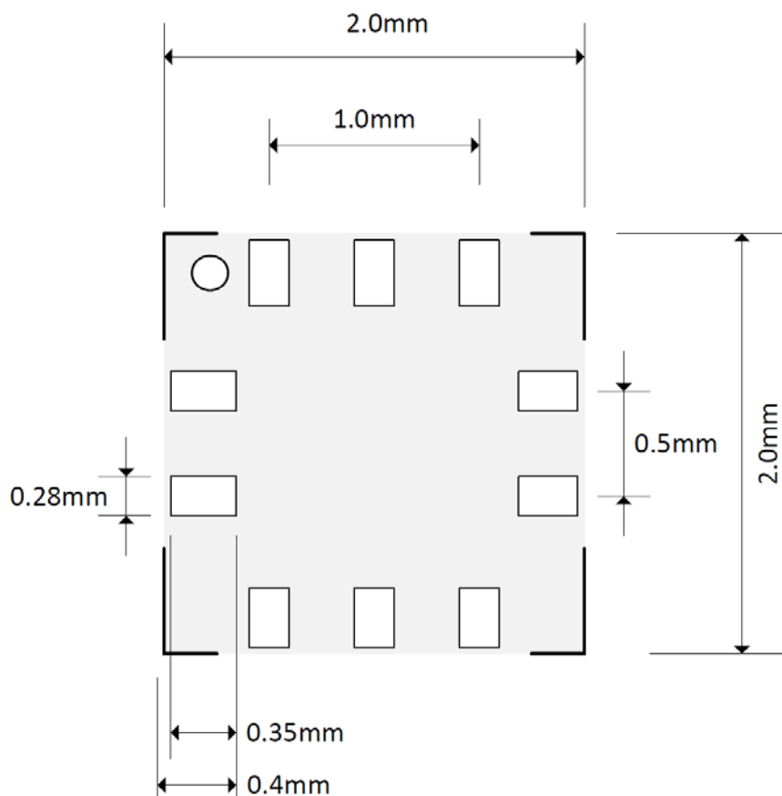
Figure 10. ICP-10100 & ICP-10101 recommended PCB land pattern
